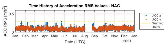
Figure 6: Exemplary evaluation of tower top vibrations according to VDI 3384. Data source: internal.
