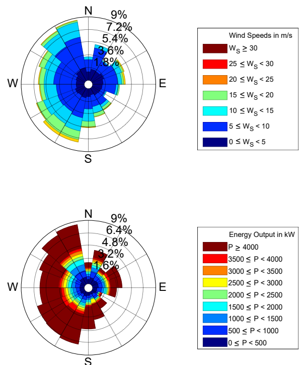
Figure 3: Exemplary analysis of wind direction distribution and energy output. Data source: internal.
